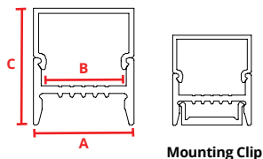
Mounting Clip
