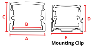
Mounting Clip
