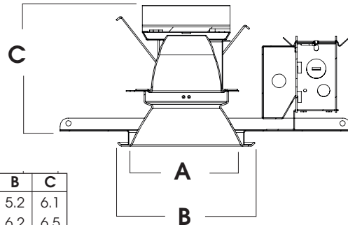
CROSS-SECTION
