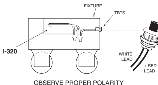
Illustration 2 Strip Fixture
